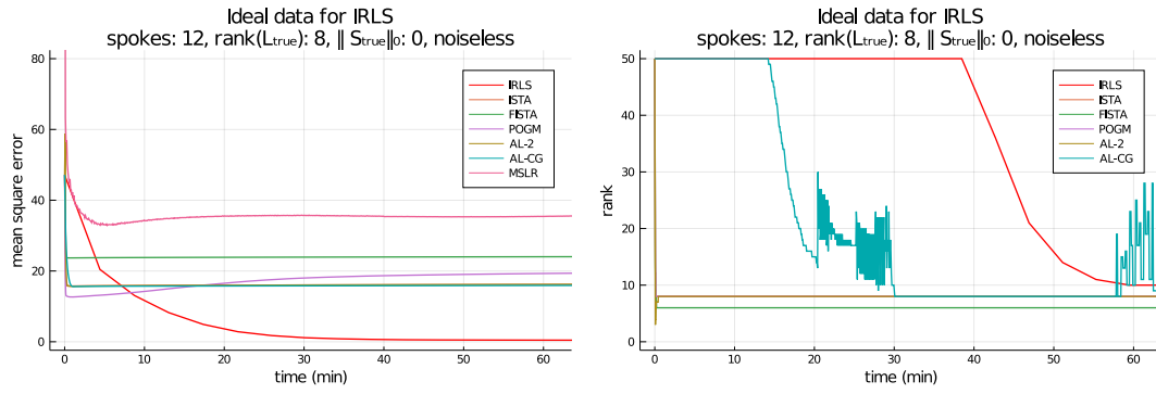
Figure 5.6: Ideal case: low-rank only and noiseless All algorithms converges and HM-IRLS gives the best, almost perfect result. Even tough HM-IRLS seems to be the slowest, in the mathematical sense, it is the fastest. Here on the image the red line shows the result of 30 iterations, while the others perform multiple thousands of iterations. On the right image, showing the rank over the iterations, one can not that HM-IRLS is more careful with decreasing the rank than other methods, and the decrease is also more smott.
