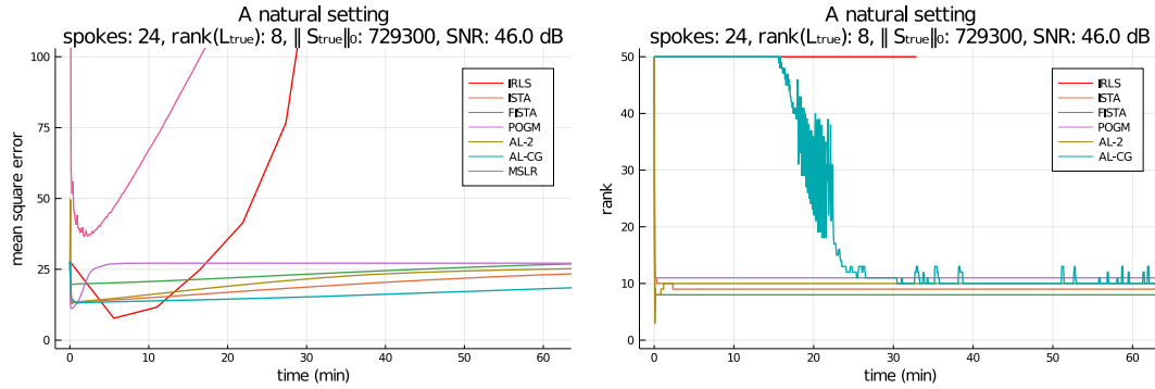
Figure 5.7: Setting that mimics the real-life settings. HM-IRLS diverges as MSLR also does.
