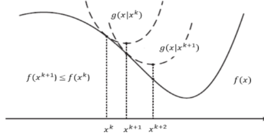
Figure 4.1: Intuition for IRLS. the IRLS scheme majorizes the cost function in the locality of the solution of the previous step by a quadratic function, and then solves for it (note that this general scheme is called majorize-minimize or MM methods). If the quadratic function is chosen appropriately, then each iteration brings closer to the solution. Source: [111].
