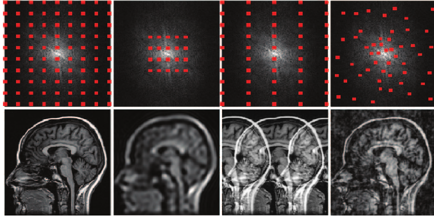
Figure 3.5: Connection between the sampling pattern and the introduced inference. Using inverse DFT replacing the missing values with zeros leads to different type of undersampling artifacts. Sampling only the center reduces the resolution, undersampled equispaced scheme adds shifted copies of the signal to the recovered image, and random sampling spreads the inference uniformly. Source: Adapted from [55].
