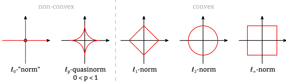
Figure 3.1: \ell_p balls in 2D.
