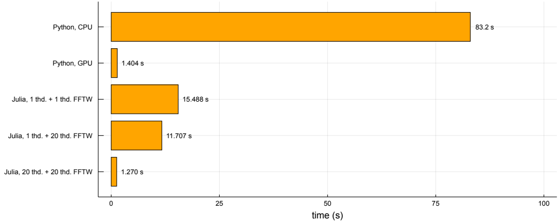
Figure 5.4: Comparison of speed different implementations for the gridding reconstruction problem (i.e. a large scale adjoint NFFT with batch dimensions).
