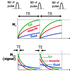
Figure 2.7: T_1 weighted sequence. Choosing the TR value to be relatively short, and TE to be relatively short, the difference due to the variation of T_1 value over tissues would dominate over differences caused by different T_2 value. Source: Adapted from [23].
