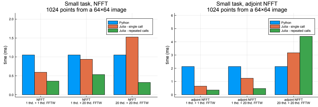
Figure 5.1: Comparison of running time between the Python implementation in SigPy package (blue), and the Julia implementations (orange: initialization and computation), green: computation only) at different threading settings in the case of a small problem (small input image with relatively few sampling points). For small images, single threaded Julia version is the fastest. (Note that the Python implementation does not implement multithreading, and hence the height of the three blue bar is the same.)
