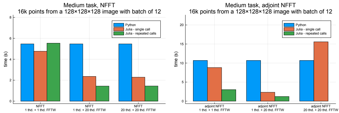
Figure 5.2: Comparison of running time in the medium sized setting: Single threaded Julia + multi-threaded FFTW yielded the best performance.
