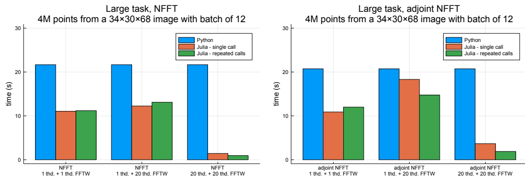
Figure 5.3: Comparison of running time in case of large number of sampling points: Multithreaded Julia code + multithreaded FFTW were the fastest.
