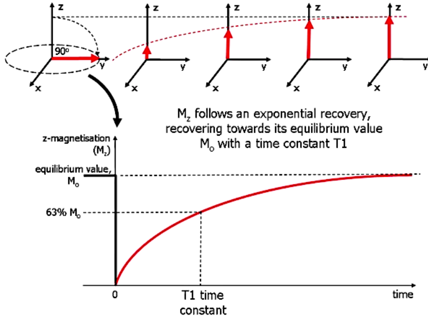
Figure 2.4: T_1 relaxation after a 90^\circ RF excitation. By the end of the pulse, the magnetization rotated from the z-direction to the x-y plane; therefore, the longitudinal component is reduced to zero, and gradually it returns to the equilibrium. Source: [23].
