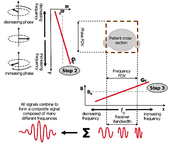
Figure 2.11: Process of phase and frequency encoding. First, a gradient along the y-direction between the RF excitation and the readout causes a gradual de-synchronization of phase along the y-axis because protons experiencing higher external field will have a higher Larmor frequency. Second, a gradient along the x-direction can be used to separate signal sources along that dimension by the difference in their frequency. Source: [23].
