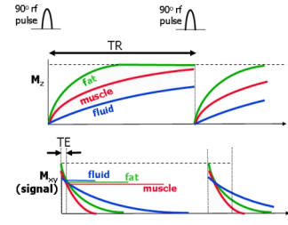
Figure 2.9: Proton density (PD) weighted sequence. Choosing the TR value to be relatively long, and TE to be relatively short, the difference due to the variation of both T_1 and T_2 values are minimized, and hence mostly the density of protons would determine signal strength. Source: Adapted from [23].
