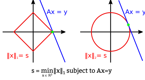
Figure 3.2: Solution of \ell_1 and \ell_2 minimization problems. Matrix \mathbf{A} \in \mathbb{R}^{1 \times 2} is an underdetermined linear system, and the task is to find \mathbf{x} \in \mathbb{R}^2 with minimal \ell_1 -norm such that it satisfies the equation \mathbf{Ax} = \mathbf{y} for fixed \mathbf{y} \in \mathbb{R} . The number of solutions are infinite (all points along the blue line), and the unique solution of minimization problem is marked with a green star. Note that \ell_1 minimization gives sparse solution, while \ell_2 minimization is not sparsity seeking.
