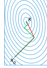
Figure 3.11: Visualization of the advantage of the CG method compared to GD: CG requires significantly fewer steps. The green line shows the path of the GD method, red shows the path of the CG method. Source: [66].
