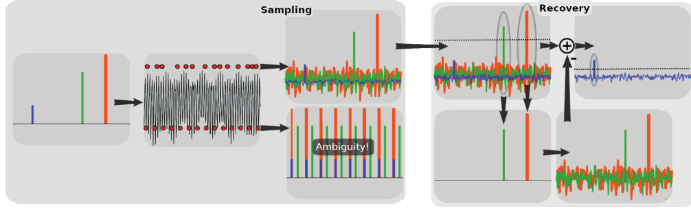
Figure 3.4: A heuristic process for reconstruction signal from randomly undersampled data. In the left block, the result of Fourier analysis is shown for both equidistant and random sampling, demonstrating the underdetermined nature of equidistant undersampling (bottom) and the noise-like effect of random sampling (top). In the right block, a simple method is applied that selects the peaks above a certain threshold as candidates, calculates the inference of these peaks, and subtracts the calculated inference from the spectrum allowing detection of further peaks after lowering the threshold. Source: Adapted from [55].
