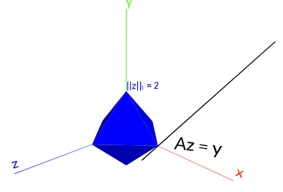
Figure 3.3: \ell_1 minimization in 3D.
