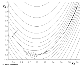
Figure 3.10: Example of the effect of inappropriate step size, "curved valley" and flat area: slow convergence of gradient descent method. Source: [65].
