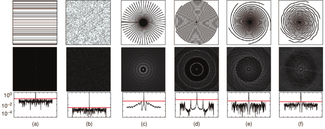
Figure 3.8: PSF of the central pixel for various sampling trajectories: (a) randomly chosen horizontal lines, (b) uniformly selected random points, (c) radial, (d) uniform spirals, (e) variable density spirals, and (f) variable density perturbed spirals. The red line marks the overall coherence level.
