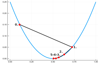
Figure 3.9: Example for backtracking algorithm. This 2D section of a high dimensional function is selected by the gradient direction, and we are looking for the local minimum along that slice. In the first step, a relatively large step size is chosen, which gets gradually decreased until local minimum is reached.
