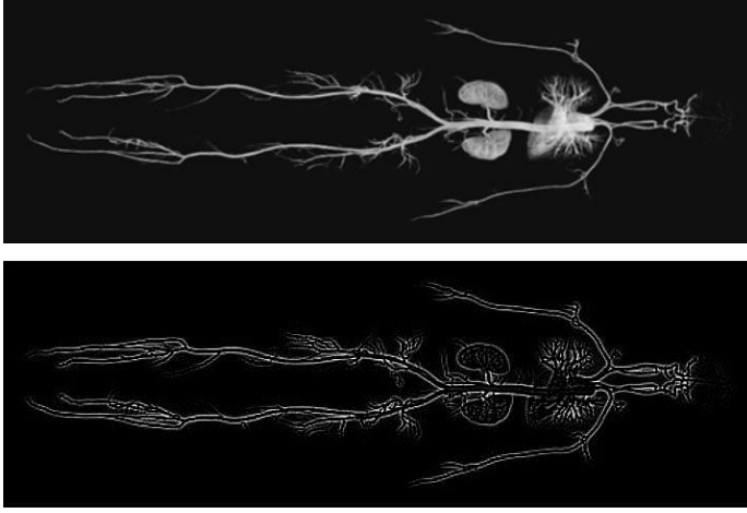
Figure 3.6: MR angiograms (MR images tuned to show blood vessels) are intrinsically sparse even in image domain (top image), but sparseness can be further improved by edge detection algorithms (bottom image) because only the morphology of the blood vessels are diagnostically relevant. Source: Adapted from [56].
