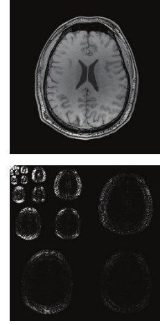
Figure 3.7: MRI images of the brain are not sparse in image domain, but they are in multiple wavelet transform domains. Source: [57].
