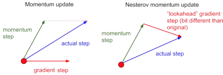
Figure 3.12: Difference between heavy ball momentum and Nesterov's momentum: While the heavy ball simply performs a weighted addition of the momentum from the previous iterations and the gradient of the current position, Nesterov's method combines these term in a counterintuitive, yet optimal manner. Source: Image is adapted from [74] and the idea of intuitive description of Nesterov's momentum rule as "lookahead" gradient step originates from [75].
