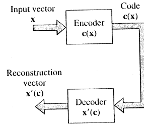
FIGURE 9.5 Encoder-decoder model.
