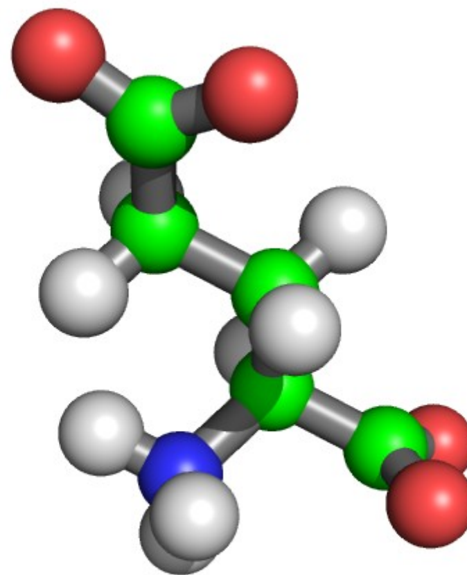
Glutamate
