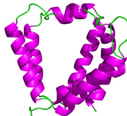
\alpha solenoid
