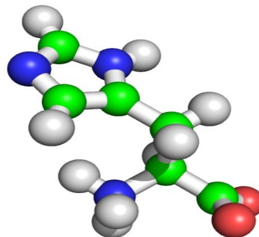
Histidine
