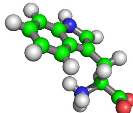
Tryptophan
