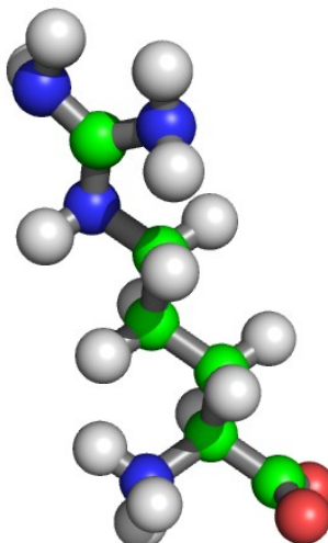
Arginine
