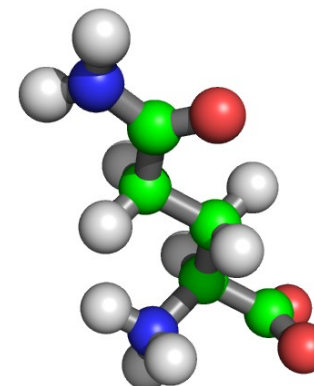
Glutamine
