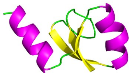
\alpha\beta\alpha sandwich
