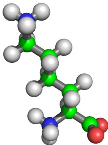
Lysine
